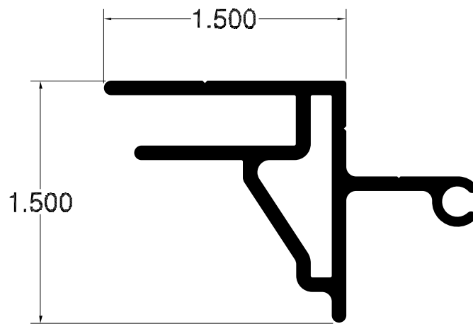
Bleed Rigid Retainer Part# 2048
